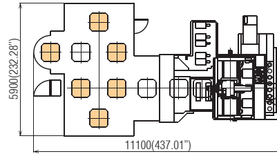
[6-pallet horizontal type with set-up station]
