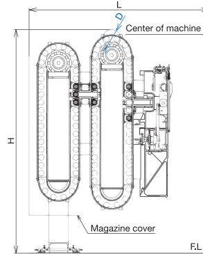
80, 116-tool capacity magazine
