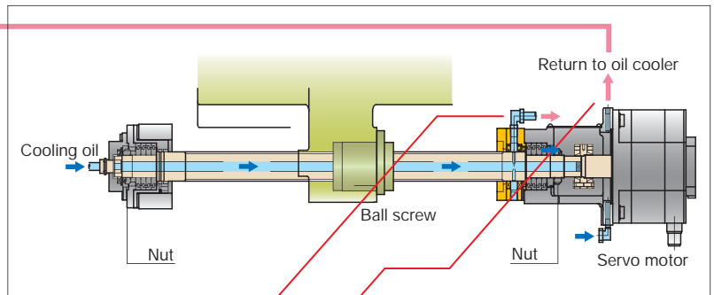
Core cooling ball screws and Double anchor pre-tension system
