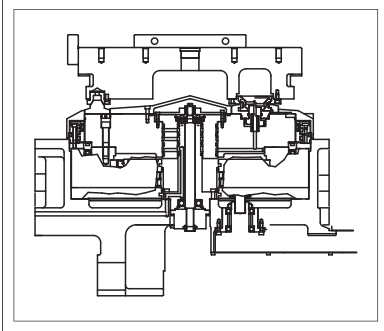
Drive with new method (HM400/HM500S, HM5100/HM6000S, HM630/HM800S)
