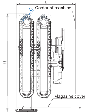
120, 156-tool capacity magazine
