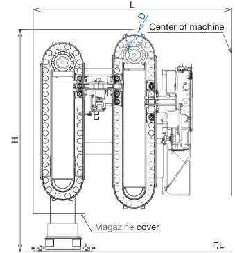
120, 176-tool capacity magazine
