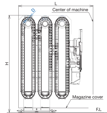
178, 232-tool capacity magazine
