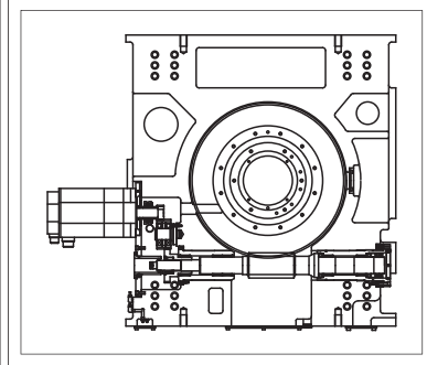
Worm and worm wheel drive (HM800/HM1000S, HM1000/HM1250S)
