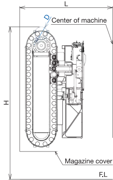
40, 60-tool capacity magazine
