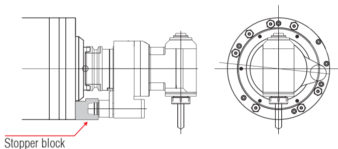
Dual-contact holder is loaded, no space between holder and spindle nose.
