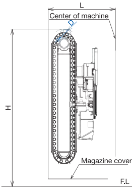
40, 60, 80-tool capacity magazine
