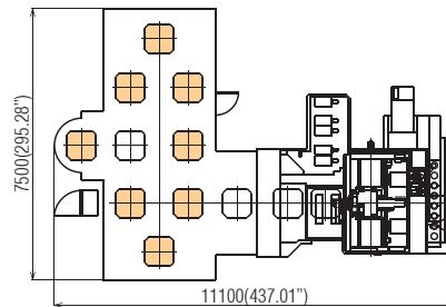
[8-pallet horizontal type with set-up station]
